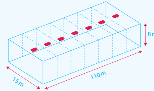
Fig. 11: Seven devices in the light colour "red" are needed to provide an alert throughout the area specified.
