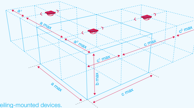
Fig. 7: Ceiling-mounted devices.
