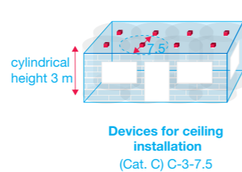
Fig. 9: Number of devices required by approval category. If the ceiling of the room were just 1 cm higher, the third variant could not be used.
