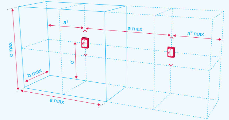
Fig. 8: Wall/pillar-mounted devices.
