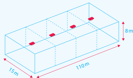
Fig. 10: Just four devices in the light colour "clear" are needed to provide an alert throughout the area specified.
