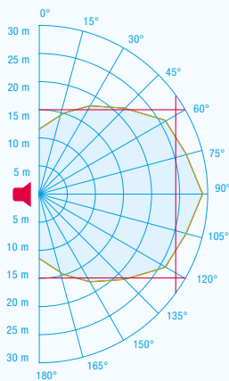
Type A signaling device, required sound level 75 dB(A), DIN tone. Smoothed area: width 25.6 m / length 26.5 m / area 678.7 m 2
