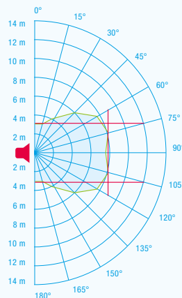
Type B signaling device, required sound level 75 dB(A), DIN tone. Smoothed area: width 6.4 m / length 7.5 m / area 48 m 2
