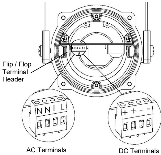
Fig. 4 Internal View of BExBGD-P 5 Joule Beacon
