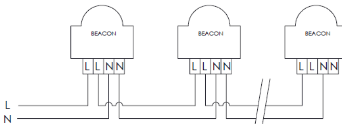
Fig. 5 AC Simplified Block Diagram
