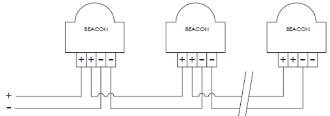
Fig. 7 DC Simplified Block Diagram (negative switching)
