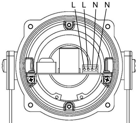
Fig. 6 AC Terminals
