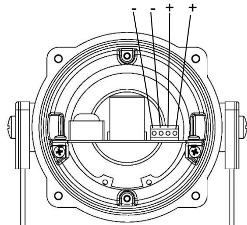
Fig. 8 DC Terminals
