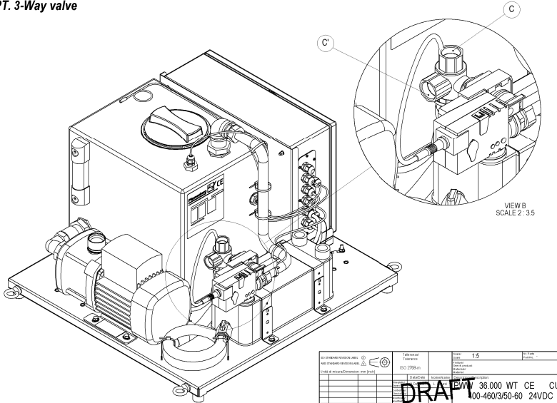
OPT. 3-Way valve
