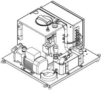
PWW 36.000 STD Plug and Play Version
