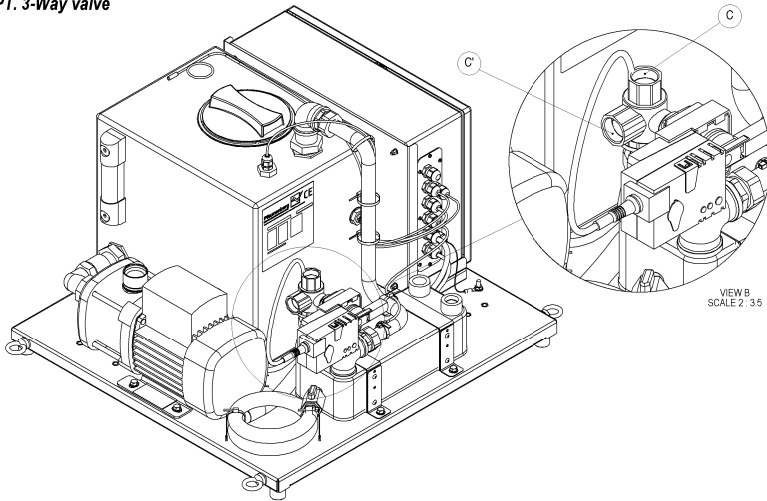
OPT. 3-Way valve
