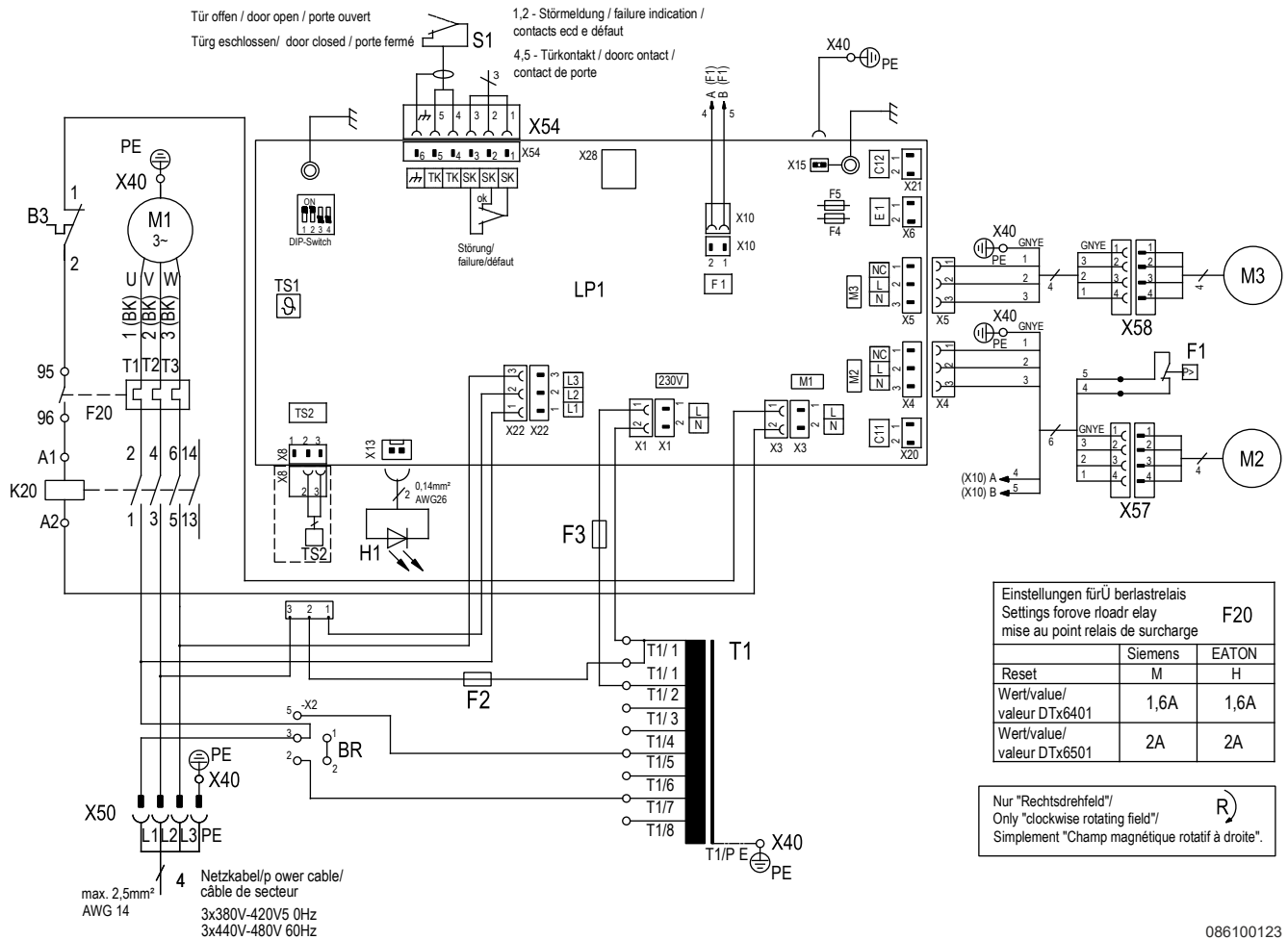
Fig. 14: Circuit diagram
