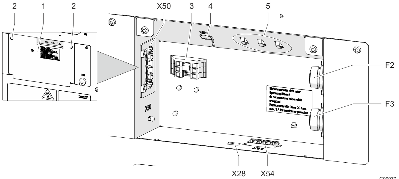
Fig. 15: Connection compartment
