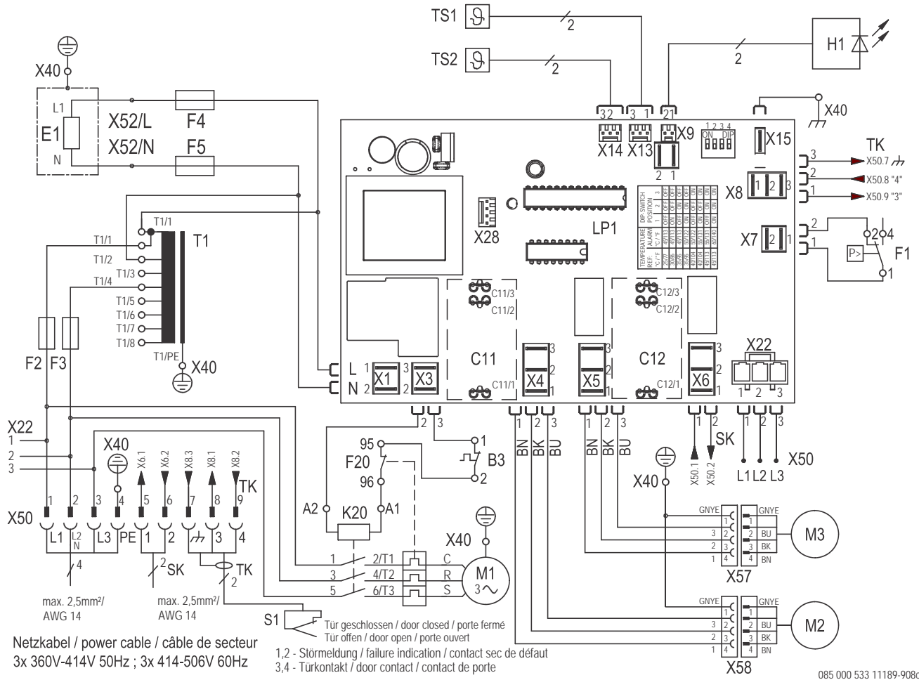
Fig. 20: Circuit diagram
